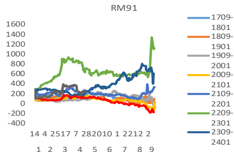
图 6: RM91 价差
